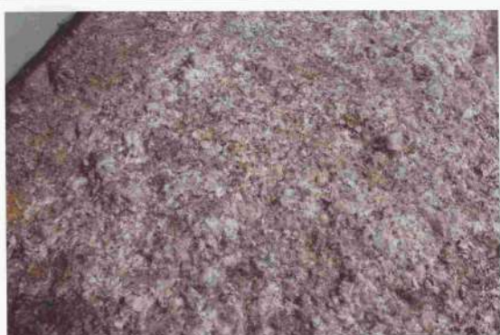
Granite. Sainte-Barbe
